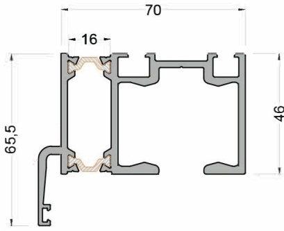
770-1301 ( 2,297 kg/mt ) FD70F03 TOP RAIL FRAME PR.
