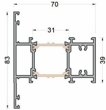
770-4101 ( 1,870 kg/mt ) FD70M01 MULLION PR.
