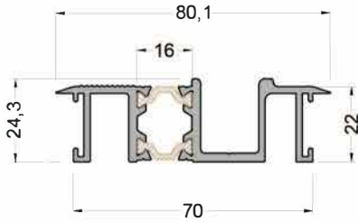
770-1201 ( 1,276 kg/mt ) FD70F02 BOTTOM RAIL FRAME PR.
